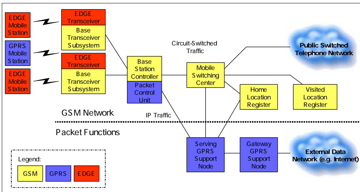
Figure 1: GSM/GPRS/EDGE Network
